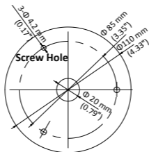
Figure 2-1 The Drill Template
